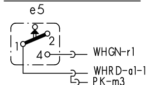
safety switch
