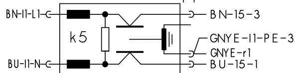
interference suppression
