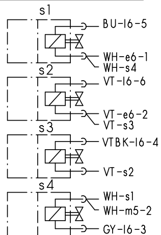
solenoid valves
