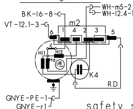
starting Relais
