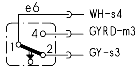
float switch
