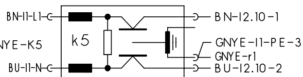
interference suppression
