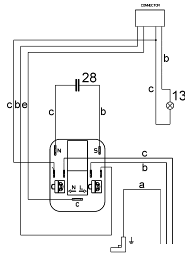
DANFOSS COMPRESSOR
