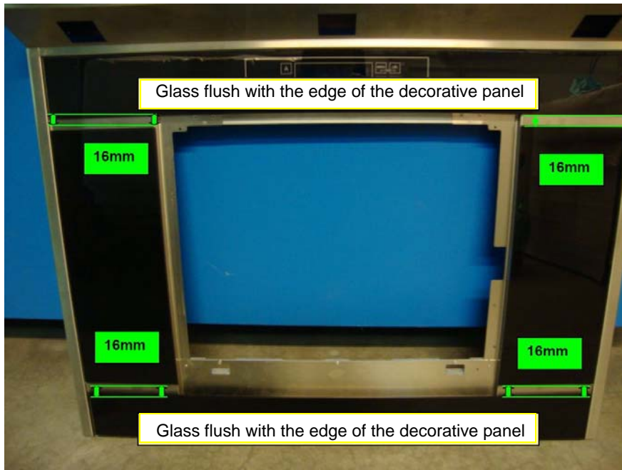
Abb. 2: Fastening the glass panel
